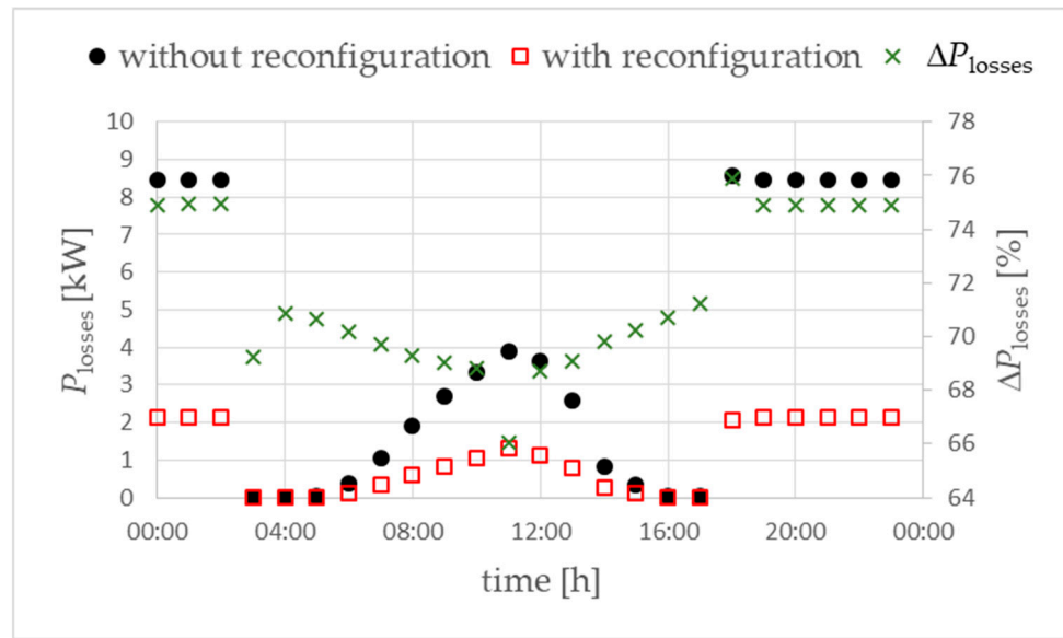
Figure 19. Active power losses in the analyzed LV network. Objective function FICR-LIc. Variant W2. \Delta P_{\text{losses}} (right vertical axis in %)—the difference in power losses “with reconfiguration” compared to “without reconfiguration”.
