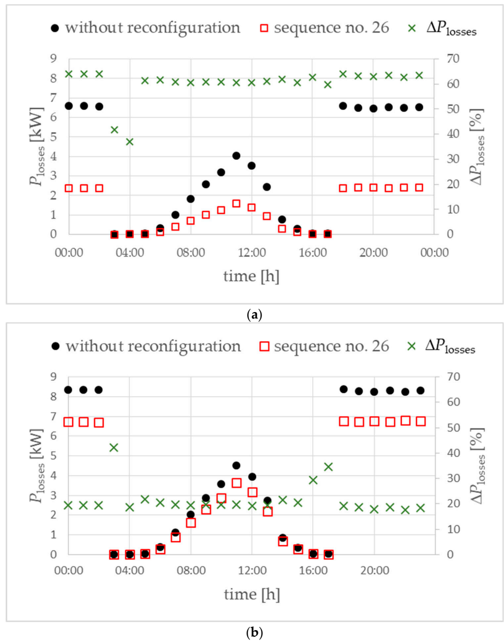
Figure 26. Active power losses in the analyzed LV network for variant W1 (a) and variant W2 (b). Objective function of DMCR-MIs. \Delta P_{\text{losses}} (right vertical axis in %)—the difference in power losses “with reconfiguration” compared to “without reconfiguration”.
