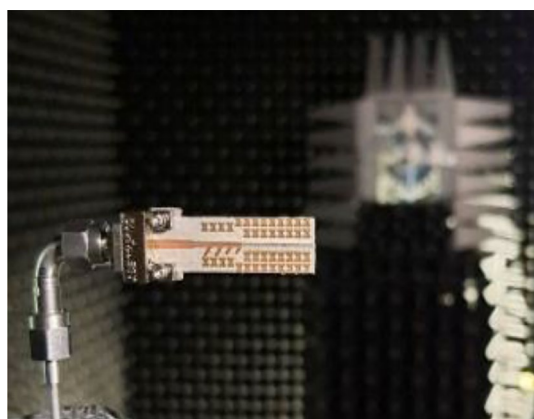
Figure 10. The radiation pattern measurement setup.
