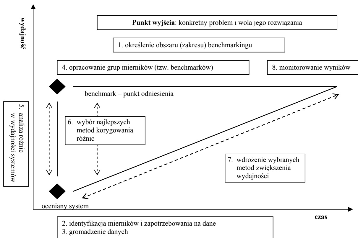
Rys. 1. Procedura benchmarkingu
