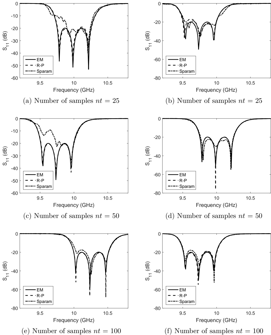
FIGURE 6.2: Comparison between residue-pole surrogate model (R-P) and scattering parameters surrogate models (Sparam) and corresponding full-wave (EM) model responses.
