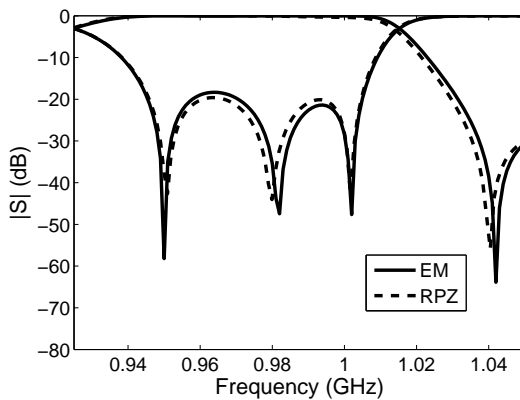
(e) f_0 = 0.975 GHz, f_z = 1.042 GHz, fbw = 0.06
