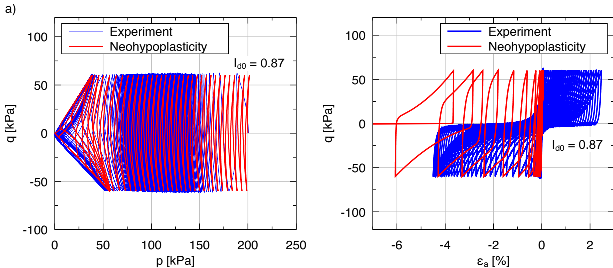
Figure 17: Isotropic consolidated cyclic undrained triaxial test with a stress amplitude of \Delta q = 50 kPa: experimental results [36, 41] vs. calculations with NHP: a) stress path in p - q diagram and b) deviator stress q as a function of axial strain \varepsilon_a .
