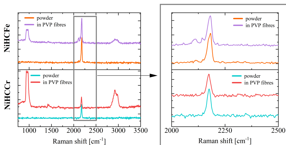
Fig. 6. Raman spectra of composite fibres of NiHCM-PVP and NiHCM bulk sample. On the right: enlargement of Raman spectra in the \nu(\text{CN}) region.
