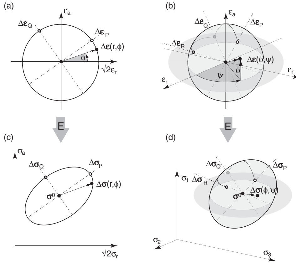
Figure 13: Isotropic elastic relation \dot{\sigma}(\sigma^0, \dot{\epsilon}) : a) axisymmetric \sigma^0 and co-axisymmetric strain increments \Delta\epsilon b) diagonal \sigma^0 and coaxial \Delta\epsilon c) stress response \Delta\sigma for (a) d) stress response \Delta\sigma for (b)
