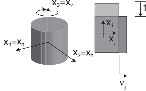
Figure 4: Axes for cross-anisotropy and the definition of the indexed Poisson number \nu_{ij}
