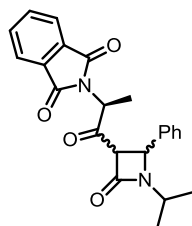
2-(1-(1-izopropyl-2-okso-4-fenyloazetyldyn-3-ylo)-1-oksopropan-2-ylo)izoindolino-1,3-dion, (98, schemat 61)
