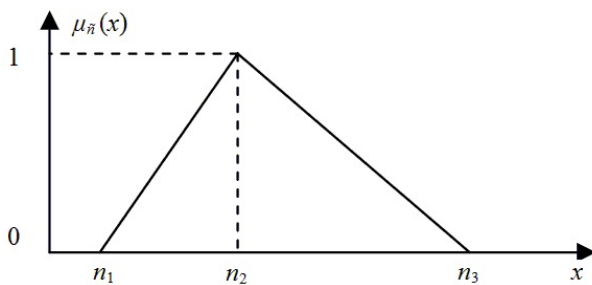
Fig. 2: Triangular fuzzy number \tilde{N} .
