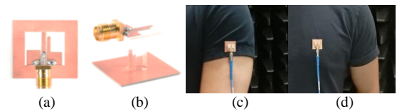
Fig. 6. Antenna prototype and characterization: (a) Front view (b) perspective view (c) On-arm (d) On-chest.
