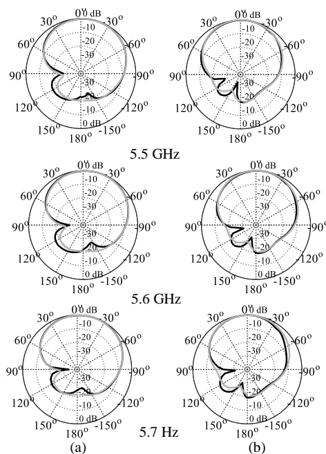
Fig. 10. Simulated (gray) and measured (black) radiation pattern of the proposed antenna in (a) the xz -plane, and (b) the yz -plane. RHCP and LHCP showed using solid and dashed lines, respectively.
