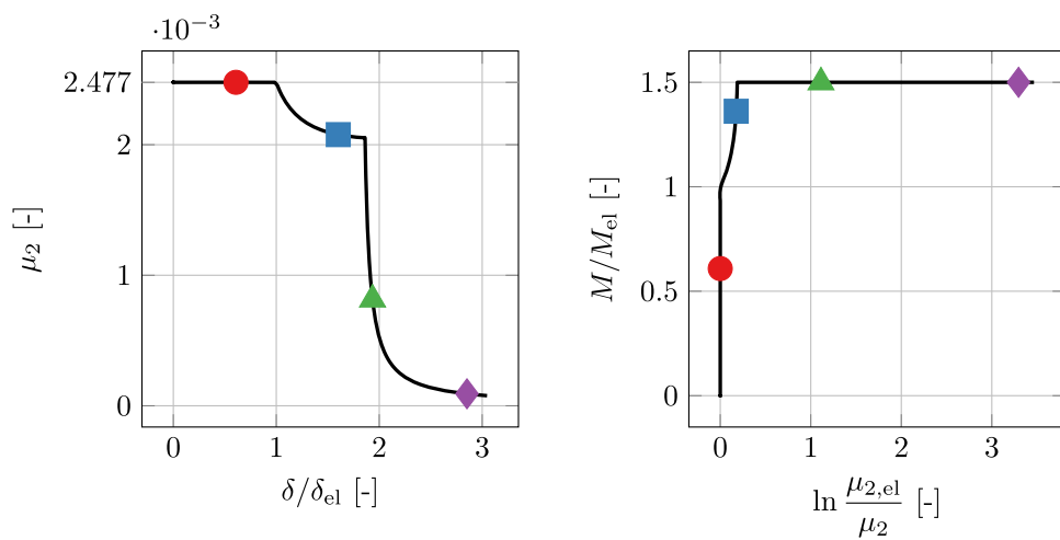
Fig. 5 Development of the diagnostic indicator (left) and bending moment (right) as a function of displacement and indicator ratios for the case of uniformly distributed load
