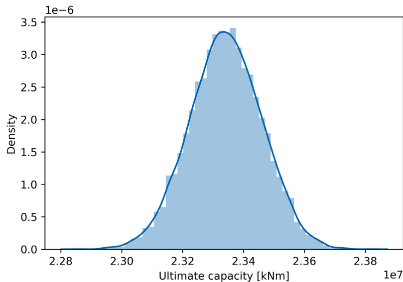
Fig. 15. Histogram of ultimate strength capacity, fully probabilistic corrosion model (model 5), hogging condition, VLCC tanker case.
