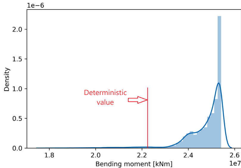
Fig. 13. Comparison of ultimate strength capacity: deterministic and probabilistic approach, collision-induced damage, hogging condition, VLCC tanker case.
