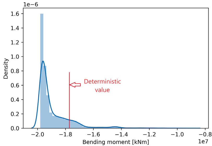
Fig. 12. Comparison of ultimate strength capacity: deterministic and probabilistic approach, grounding-induced damage, sagging condition, VLCC tanker case.
