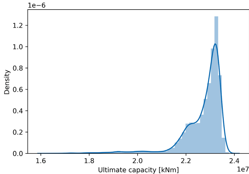
Fig. 16. Histogram of ultimate strength capacity, VLCC tanker, hogging condition, collision damage.
