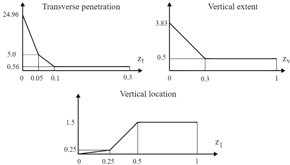
Fig. 2. Probability functions to characterize the damage extent on a ship's hull due to collision: transverse penetration, vertical extent, and vertical location.
