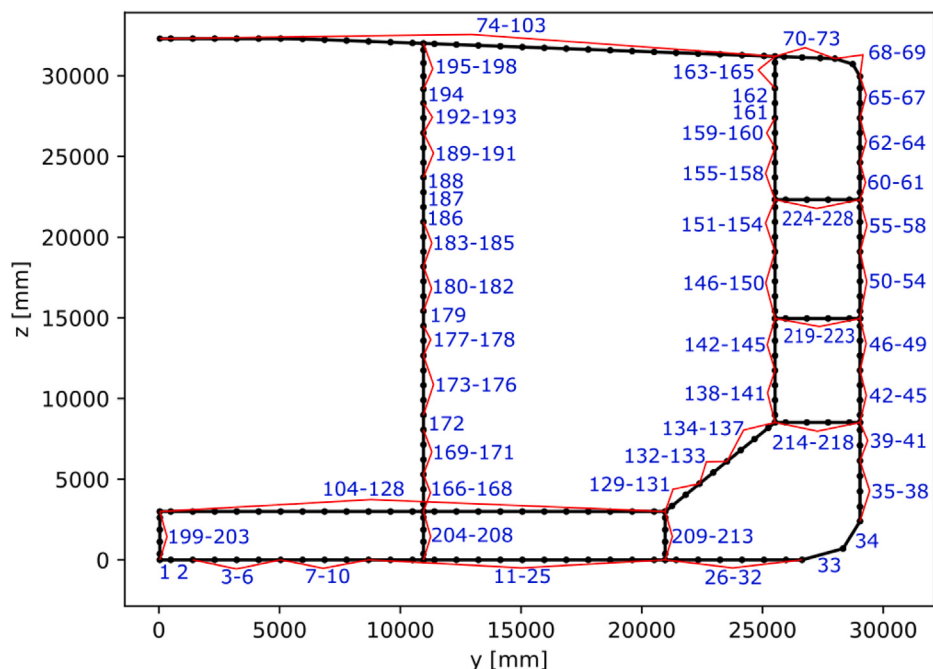
Fig. 7. Cross-section of VLCC tanker ship applied in the case study.
