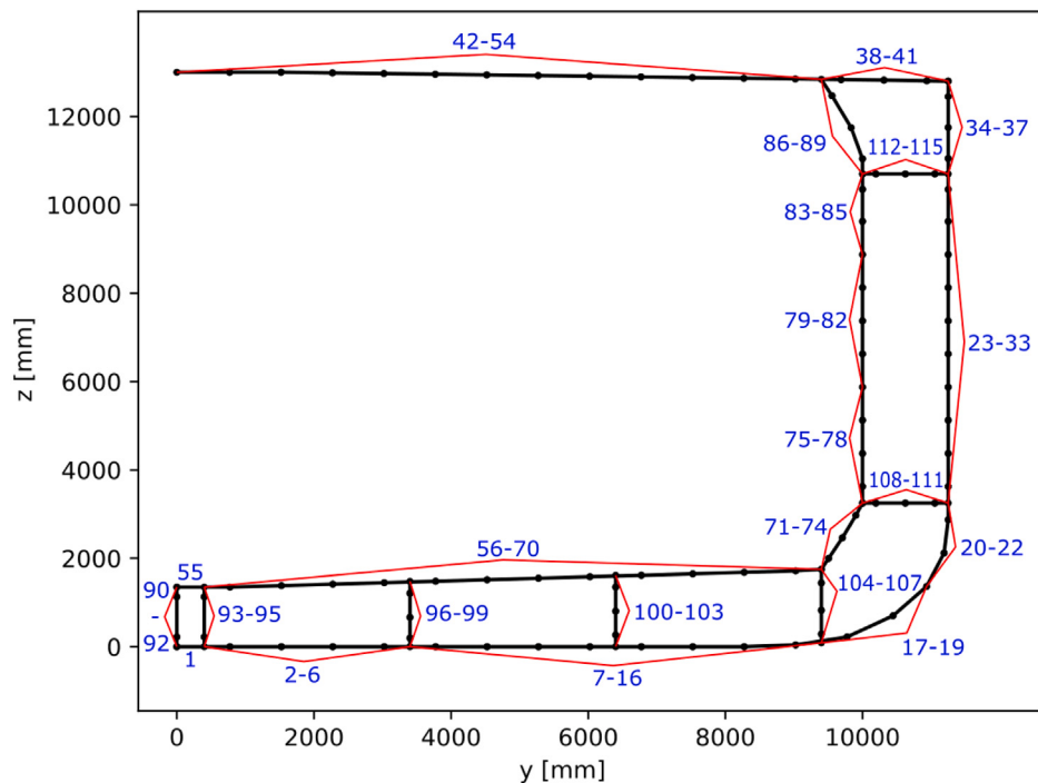
Fig. 8. Cross-section of Handysize tanker ship applied in the case study.
