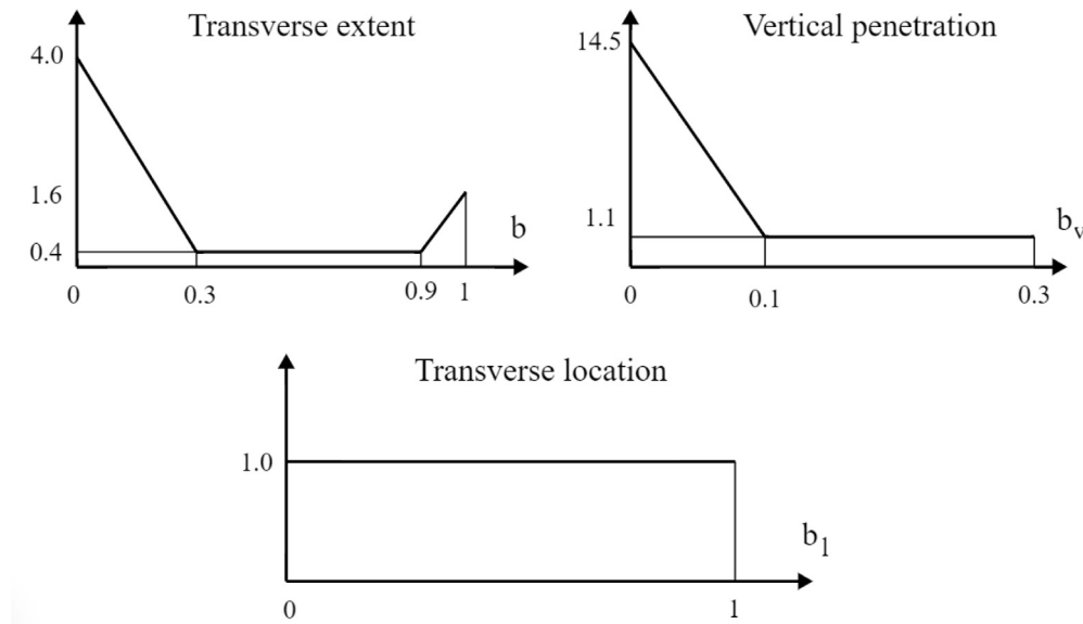
Fig. 3. Probability functions to characterize the damage extent on a ship's hull due to grounding: transverse extent, transverse location, and vertical penetration.
