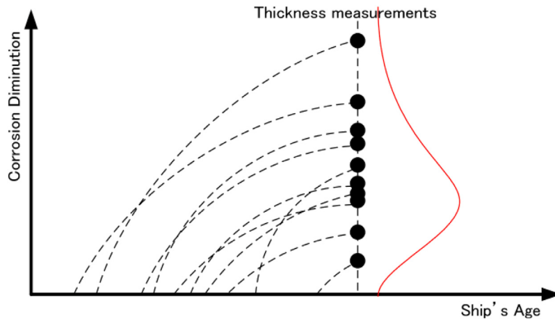
Fig. 5. Corrosion diminution within the ship hull cross-section after 25 years of exploitation based on measurements modelled as log-normal distribution [80].
