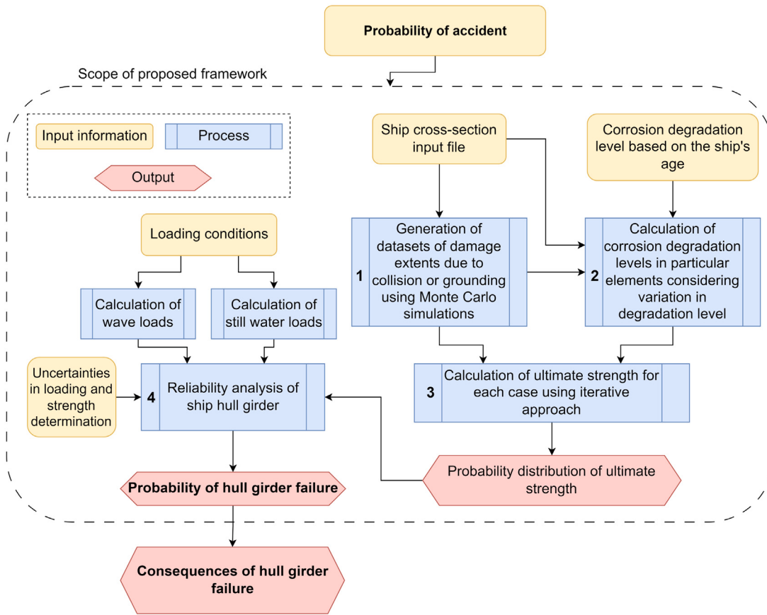
Fig. 1. Block scheme of the presented framework for hull girder failure probability assessment for accidental damage considering corrosion effects.
