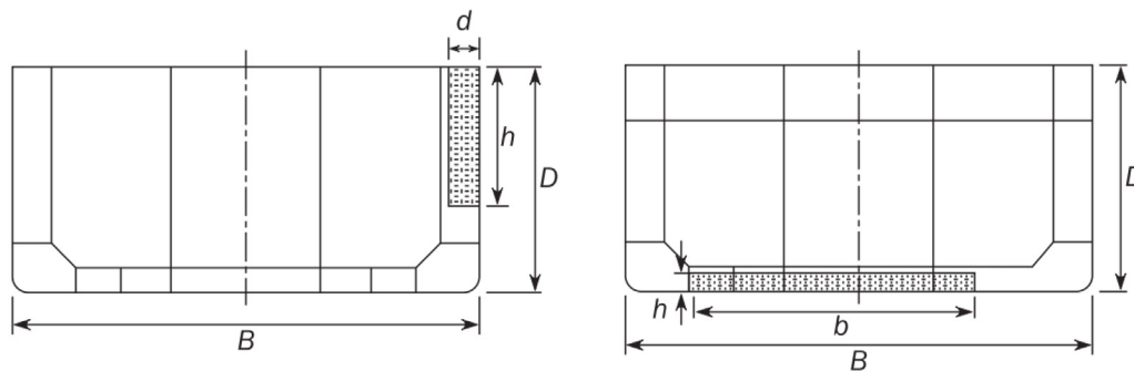
Fig. 9. Accidental damage extent due to collision (left) and grounding (right) [73].
