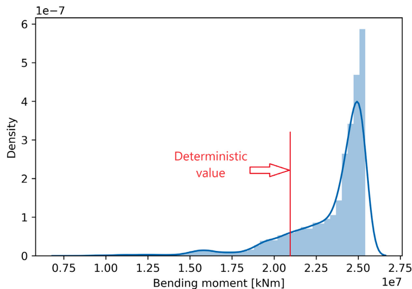
Fig. 14. Comparison of ultimate strength capacity: deterministic and probabilistic approach, grounding-induced damage, hogging condition, VLCC tanker case.
