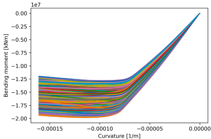
Fig. 10. Moment-Curvature relationships for probabilistic simulations considering collision-induced damage, sagging condition, VLCC tanker case.
