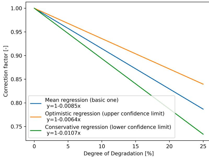
Fig. 4. Correction factor to account for the reduction in ultimate strength of a structural element considering corrosion impact in relation to the Degree of Degradation, based on [52].
