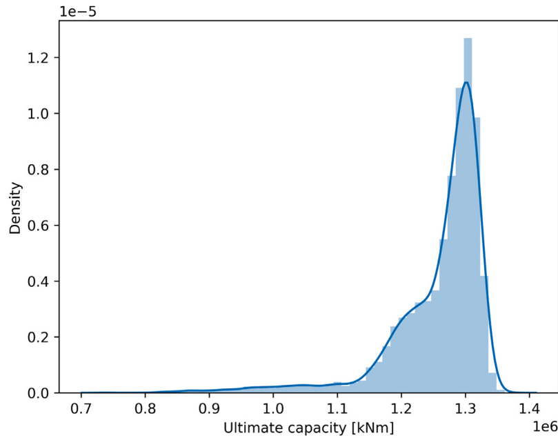
Fig. 17. Histogram of ultimate strength capacity, Handysize tanker, hogging condition, collision damage.
