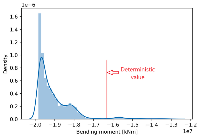
Fig. 11. Comparison of ultimate strength capacity: deterministic and probabilistic approach, collision-induced damage, sagging condition, VLCC tanker case.
