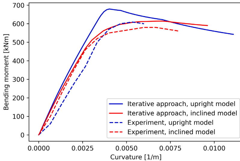
Fig. 6. Comparison between iterative approach implemented in our framework with experimental results of damaged sections presented in [82].
