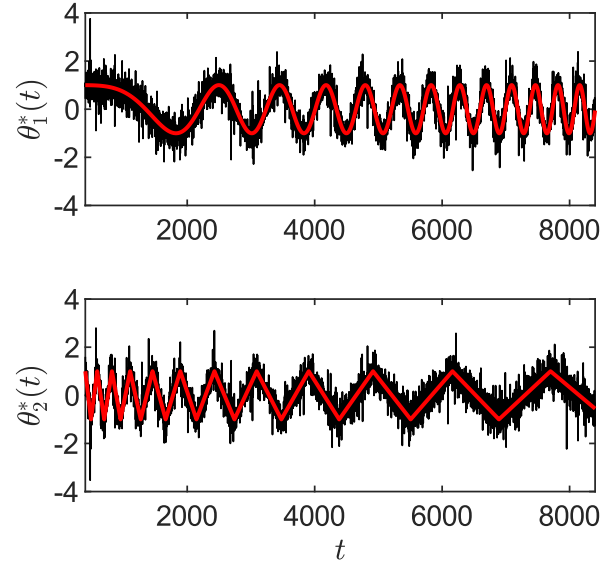
Fig. 1. Preestimated parameter trajectories of a nonstationary two-tap finite impulse response system (SNR=25 dB). Preestimates (black lines) are superimposed on true parameter trajectories (red lines).
