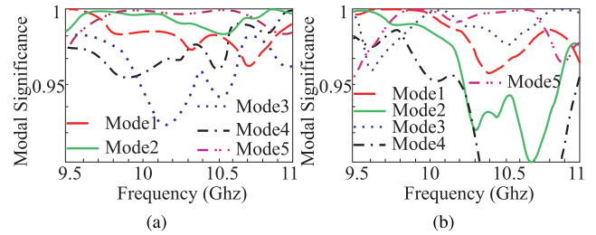
FIGURE 8. Modal significance of the 2 × 2 MS-based MIMO array: (a) without cross-shaped slot in the ground, (b) with cross-shaped slot in the ground.
