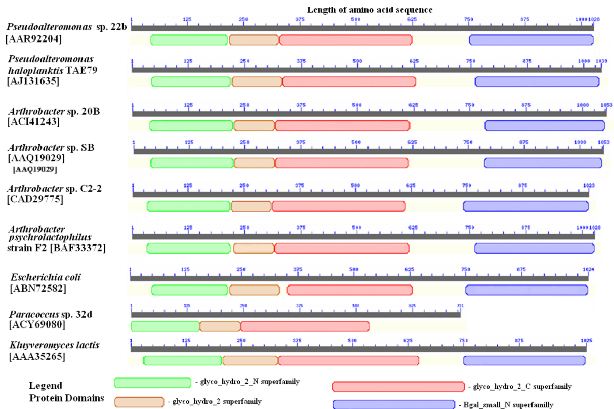
Figure 2 Topographic presentation of Pfam domains for selected LacZ β-D-galactosidases and Paracoccus sp. 32d β-D-galactosidase BgaL. The domains presented were suggested by the Pfam database http://www.sanger.ac.uk/software/Pfam and are indicated by different colors. The numbers in parentheses are the GenBank accession numbers.
