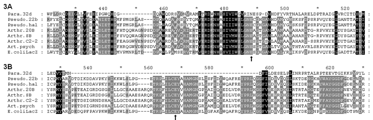
Figure 3 Alignment of the amino acid sequences of β-D-galactosidase (A) acid-base active sites, and (B) the consensus nucleophilic region of the selected LacZ enzymes and Paracoccus sp. 32d β-D-galactosidase. The numbers in parentheses are GenBank accession numbers. Proposed active site glutamic acid residues are indicated by the black arrows. Para.32d - Paracoccus sp. 32d BgaL (ACY69080), Pseudo.22b - Pseudoalteromonas sp. 22b LacZ (AAR92204), Pseudo.hal - Pseudoalteromonas haloplanktis TAE79 LacZ (AJ131635), Arthr. 20B - Arthrobacter sp. 20B LacZ (ACI41243), Arthr. SB - Arthrobacter sp. SB LacZ (AAQ19029), Arthr.C2-2 - Arthrobacter sp. C2-2 LacZ (CAD29775), Art. psych - Arthrobacter psychrolactophilus strain F2 LacZ (ABN72582) and E.coliLacZ - E. coli LacZ (ABN72582).
