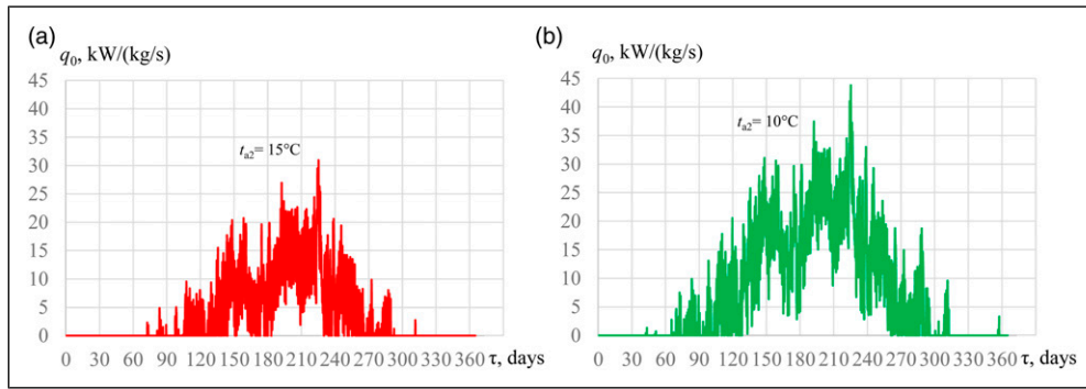
Figure 1. Changes in specific cooling capacities q_0 during 2017: (a) – q_{0,15} for t_{a2} = 15^\circ\text{C} ; (b) – q_{0,10} for t_{a2} = 10^\circ\text{C} .
