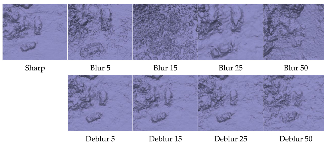
Figure 9. Solid model—visual comparison of the product part developed using photos with a varying blur kernel and their corresponding product, after the application of the method.
