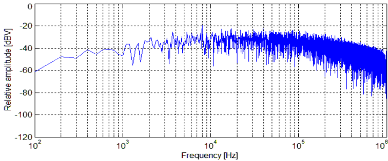
Fig. 13. The spectrum of a signal generated for reseed values of LFSR using the application written in AVR Assembler.
