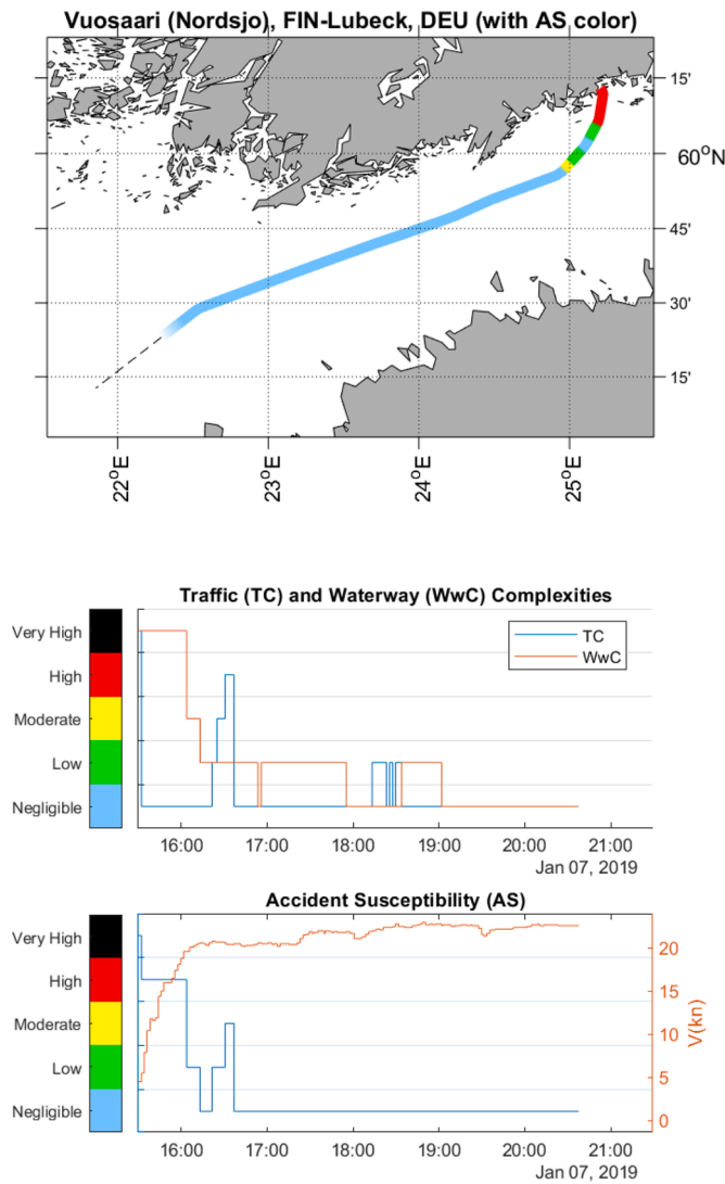
Fig. 24. Close-up of the legs of the voyage from Vuosaari (Finland) to Lubeck (Germany) located in the Gulf of Finland, including departure from Vuosaari. High traffic and waterway complexity at departure and low otherwise, make accident susceptibility high at the initial stage of voyage, subsequently dropping to low and negligible in the remaining part of the voyage. Along with the values of accident susceptibility index ship speed is depicted.
