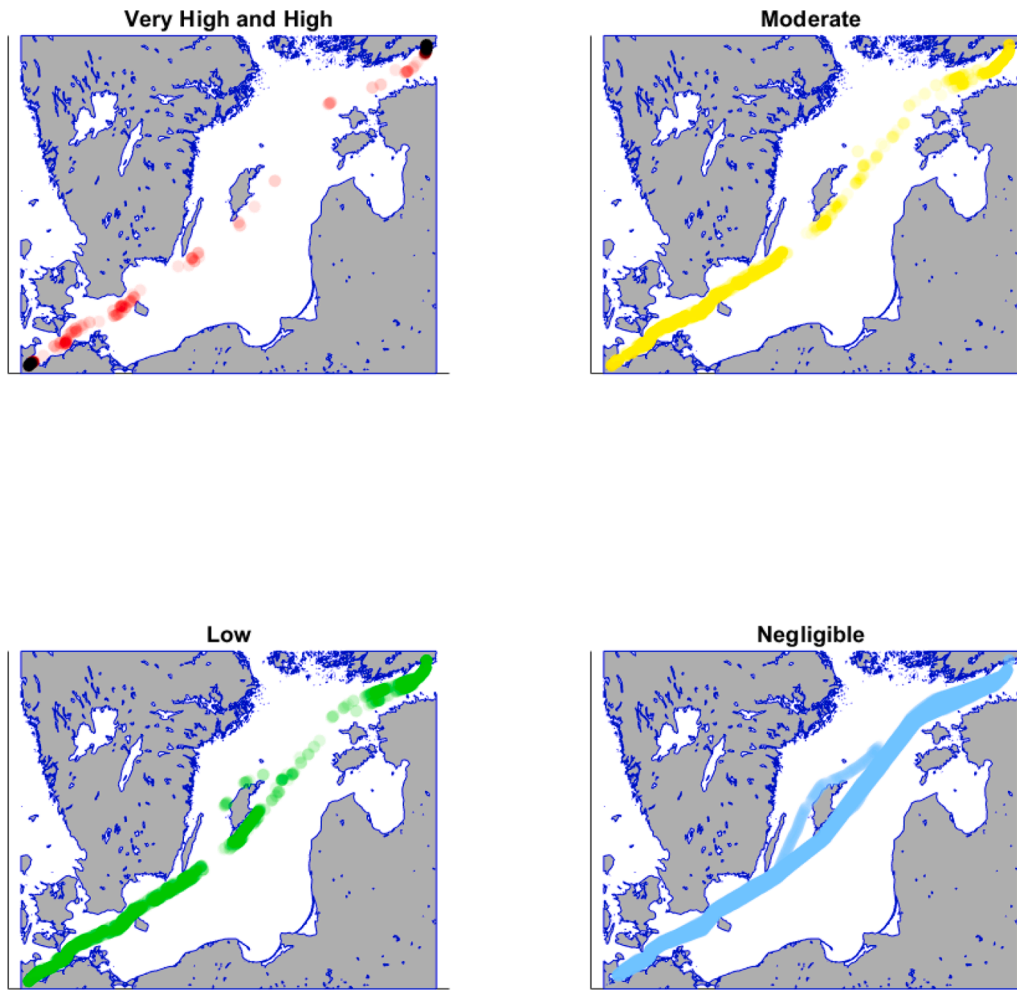
Fig. 26. Breakdown of accident susceptibility levels for the analyzed RoPax route covering 8 months (January–August) of 2019.
