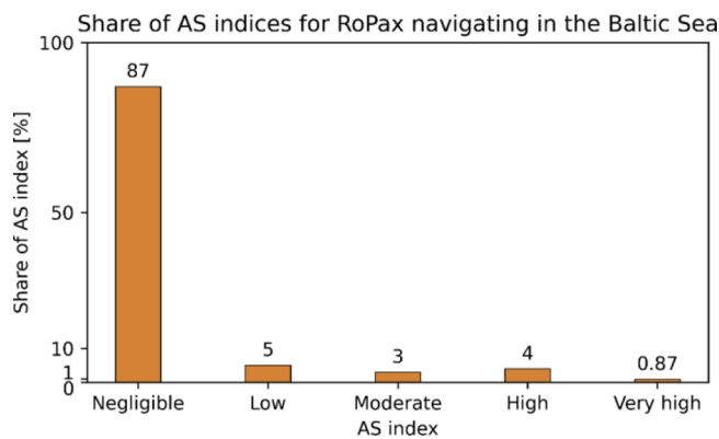
Fig. 27. Distribution of the accident susceptibility indices for the analyzed RoPax.
