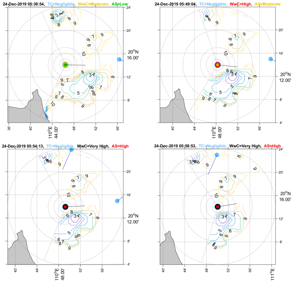
Fig. 17. Own ship navigates close to shallow water. Waterway Complexity develops from Moderate (shallow ground on starboard between 2 and 3 NM and on portside over 3NM) to Very High (shallow ground closer than 1NM away) (For interpretation of the references to color in this figure, the reader is referred to the web version of this article.).
