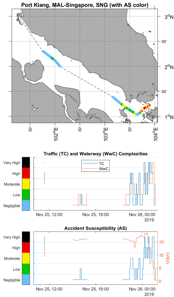
Fig. 22. Voyage from Malaysia to Singapore, with high traffic and waterway complexity on arrival: the upper image shows the track of the voyage with colors indicating Accident Potential, the dashed line shows a gap in the AIS data longer that 40 min. Below, two-time histories show Traffic and Waterway Complexities and Accident Susceptibility Index. In the time history of ASI also the ship speed is shown. No values are shown for gaps in AIS data.
