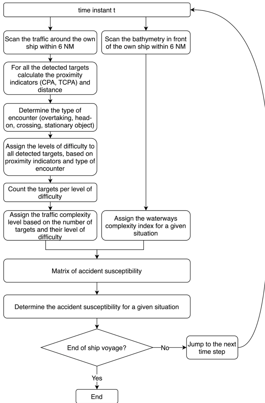
Fig. 4. Flowchart demonstrating process of accident susceptibility assessment.
