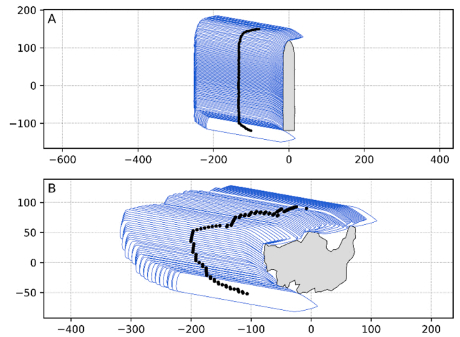
Fig. 6. The initial positioning of ship hull projections at the beginning of the simulation for a single heading, the obstacles are coloured in gray.
