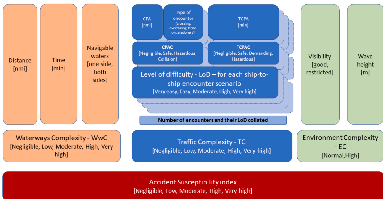
Fig. 2. Framework for accident susceptibility assessment for a ship in operation.
