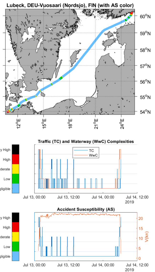
Fig. 25. Summer time voyage from Lubeck (Germany) to Vuosaari (Finland), with high traffic and waterway complexity at departure and arrival. The upper image shows the track of the voyage with colors indicating Accident Susceptibility, the dashed line shows a gap in the AIS data longer than 40 min. In the lower image, two time histories show Traffic and Waterway Complexities and Accident Susceptibility Index. In the time history of ASI also the ship speed is shown. No values are shown for gaps in AIS data.
