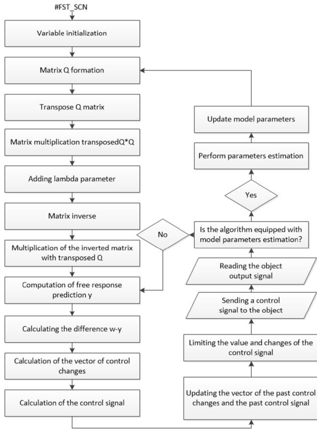
FIGURE 7. Algorithm divided into individual steps.
