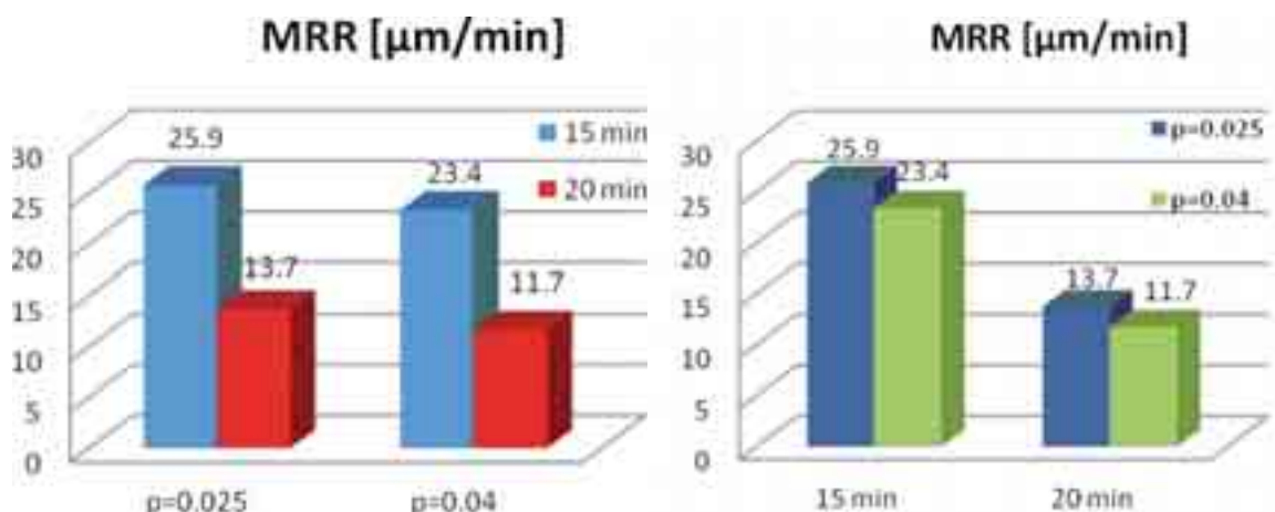
Fig. 9. Test results of MRR in μm/min depending on lapping pressure
