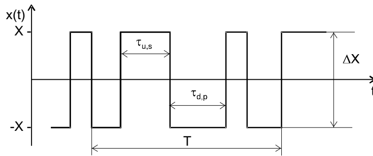
Fig. 1. Typical two-level RTS noise; \tau_{u,s} – the s^{\text{th}} duration of an impulse in the up time, \tau_{d,p} – the p^{\text{th}} duration of an impulse in the down time, \Delta X – the amplitude of RTS noise, T – observation time.
