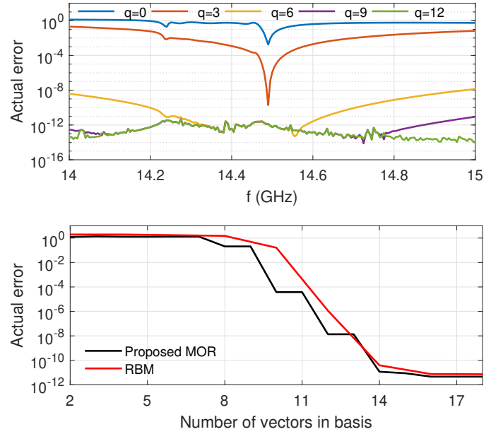
Fig. 8. Folded waveguide filter. Actual reduction-error as a function of ROM size, where q is the number of FOM eigenvectors associated with impedance zeros in the projection basis. The number of poles in the projection basis is 6.
