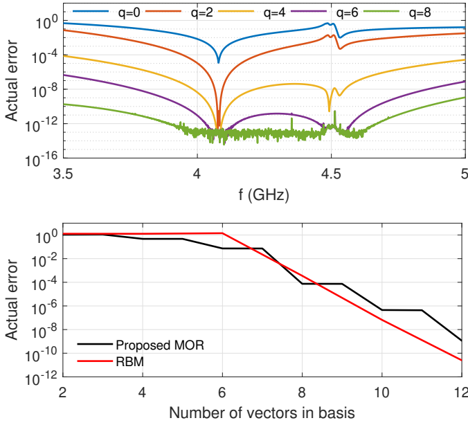
Fig. 6. Dielectric resonator filter. Actual reduction-error as a function of ROM size, where q is the number of FOM eigenvectors associated with impedance zeros in the projection basis. The number of poles in the projection basis is 4.
