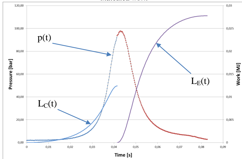
Fig.5 Dependence of work and pressure during compression and expansion strokes. L_E(t) – expansion work until the t moment, t \in \left[\frac{t_{1ob}}{2}, t_{1ob}\right] , L_C(t) – compression work until the t moment, t \in \left[0, \frac{t_{1ob}}{2}\right]
