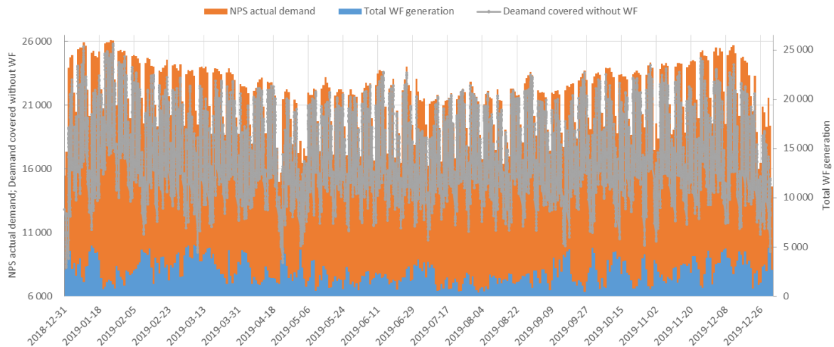
Figure 2: Coverage of electricity demand for the period from 1 January 2019 to 31 December 2019 [MW]
