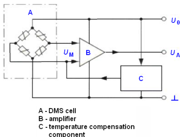
Fig.3. Thick film pressure sensor (connections)
