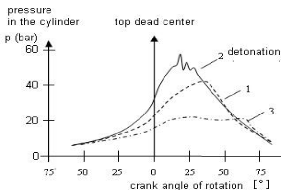
Fig.11.Dependence of rotation angle cranks and cylinder pressure
