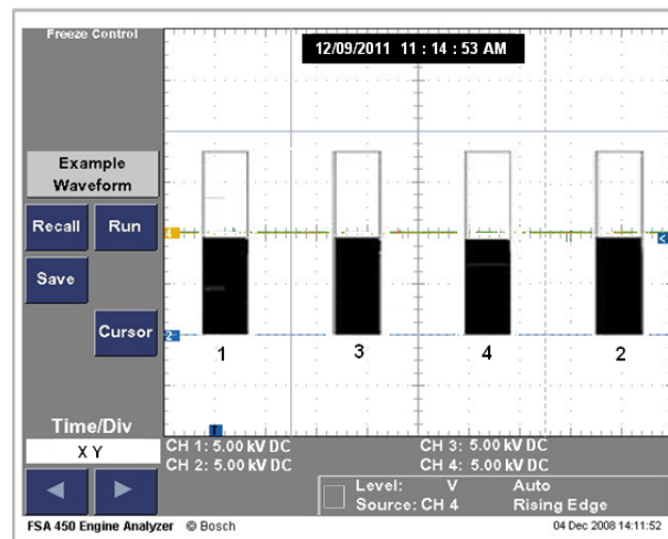
Fig.8. Graph of secondary voltage for each cylinder at idle
