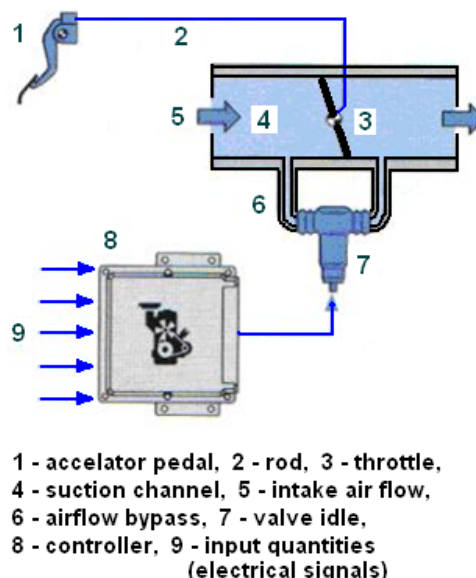
Fig.4.Principle of air control in the usual systems
