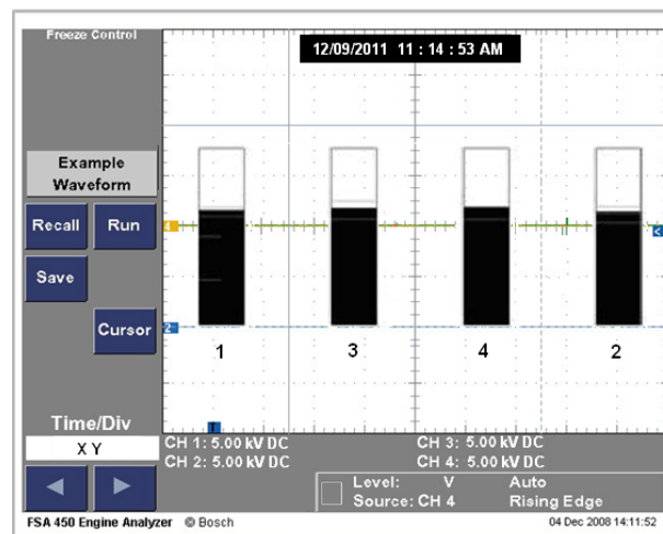
Fig.9. Graph of secondary voltage for each cylinder at higher engine speeds
