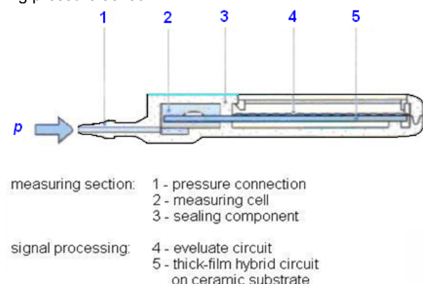
Fig.2. Thick film pressure sensor
