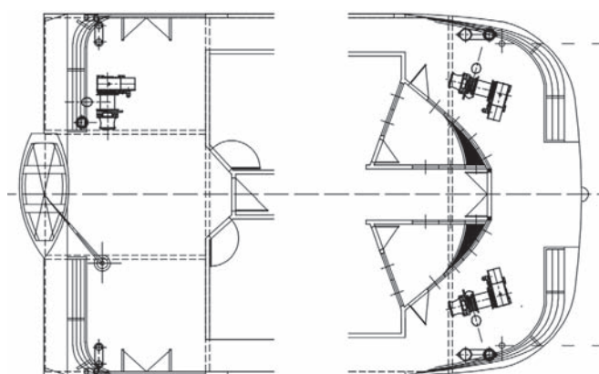
Fig.4. Example arrangement of the anchoring and mooring equipment on the pusher .
