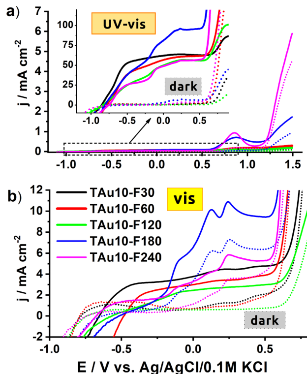
Figure 8. Linear voltammograms recorded under (a) UV–Vis and (b) Vis irradiation for laser-modified samples with initially deposited 10 nm Au film.
