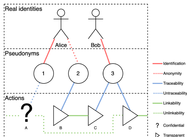
Fig. 2 Consider a scenario where Alice is an anonymous customer and Bob is a public service provider (SP). Alice controls two addresses, labelled 1 and 2. The link (shown as a red line) between Alice's real identity and address 1 has been compromised, allowing identification. However, the link to address 2 remains unknown, preserving anonymity. Alice performs two actions, A and B. Action A is from the compromised address 1, while action B is from the anonymous address 2. Action A is confidential, meaning that despite the compromised pseudonym, the nature of the action remains undisclosed. Action B is transparent, but it cannot be linked to Alice as long as the connection to pseudonym 2 remains hidden
