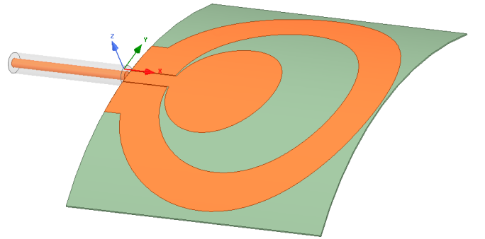
Fig. 3. HFSS model of conformal antenna
