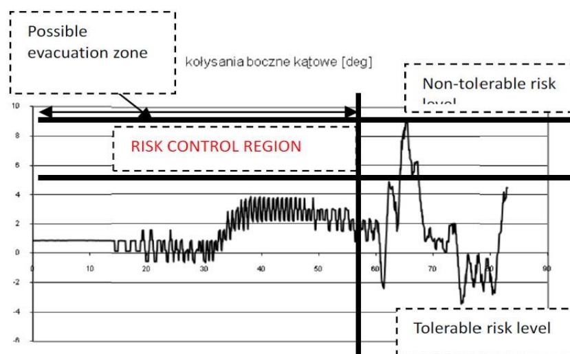
Figure 6. An example of the roll function in time domain and risk evaluation criteria applied for the assessment of safety of the container ship in abnormal/damaged conditions.
