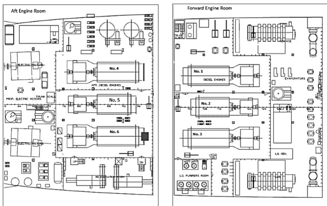
Fig. 1. Arrangement of Carnival Triumph ship power plant.
