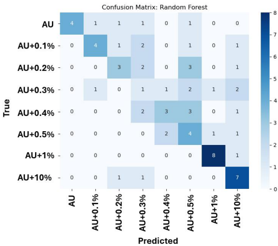
Fig. 4. Confusion matrix for Random Forest classification of glucose concentrations (0.1%–10%) in artificial urine (AU). The extended concentration range was used for exploratory evaluation of classification performance, with a focus on early detection. AU: artificial urine; AU+X%: artificial urine with X% glucose.
