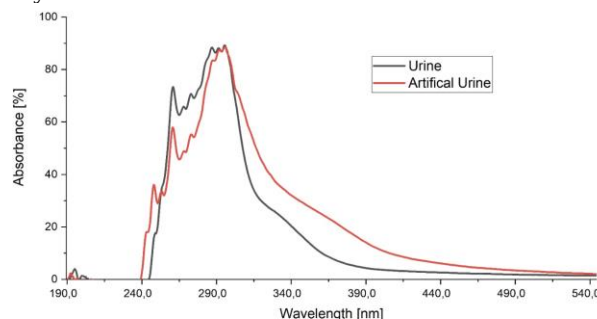
Fig. 2. Comparison of the UV-VIS spectra of human urine with those of the artificial urine used in this study.
