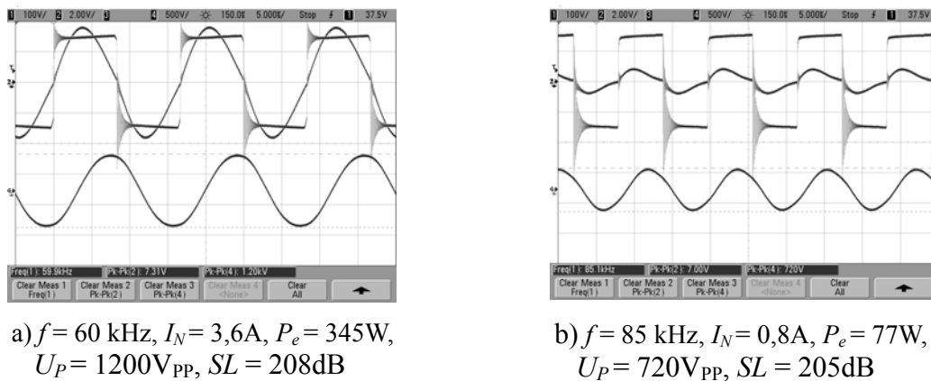
Fig.8. Voltage and current at pulse transmitter outputs with U_N = 150\text{V} , exciting a 16 element transducer module with series compensation at two ends of the working bandwidth. The bottom part of the oscillograms shows transducer voltage
