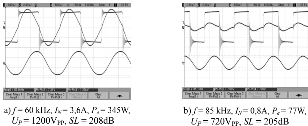
Fig.8. Voltage and current at pulse transmitter outputs with U_N=150 V, exciting a 16 element transducer module with series compensation at two ends of the working bandwidth. The bottom part of the oscillograms shows transducer voltage
