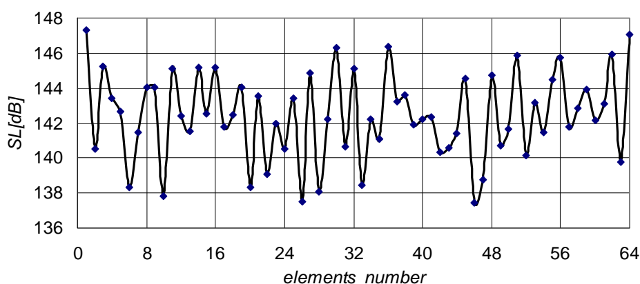
Fig.1. Spread of source level SL [dB ref. 1\mu\text{P/V/m} ] for 64 array elements
