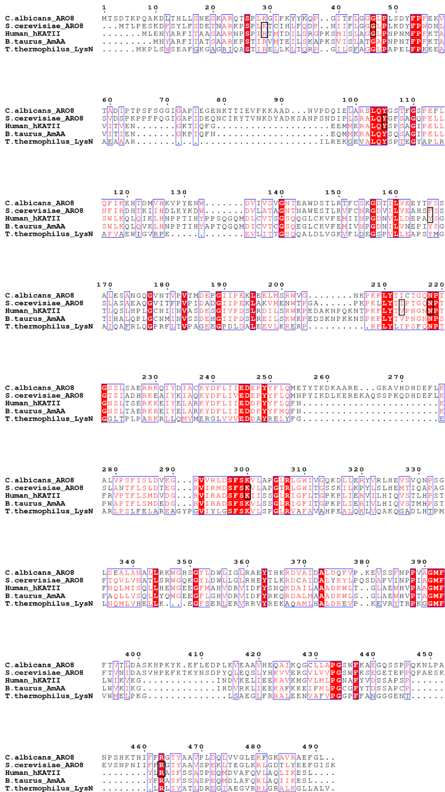
Figure 2 Multiple amino acid sequence alignment for (A) CaAro8p and (B) CaYer152Cp from Candida albicans and aminotransferases from other organisms. Highly conserved residues are marked as white letters on a red background, similarities are marked in red, the most important residues participating in substrate and PLP binding in hKATII and ScAro8p are marked in bold black frame (Rossi et al. , 2008; Han et al. , 2009; Bulfer et al. , 2013). ClustalW (Larkin et al. , 2007) was used to perform a multiple sequence alignment and ESPrnt (Robert & Guet 2014) was used to produce the figure.
