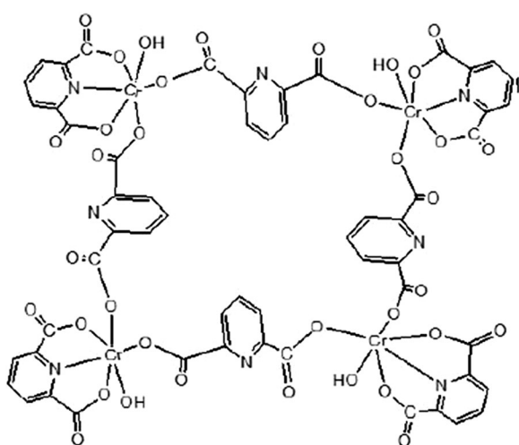
Fig. 4 The proposed structure related to formation of the Cr-MOF sorbent
