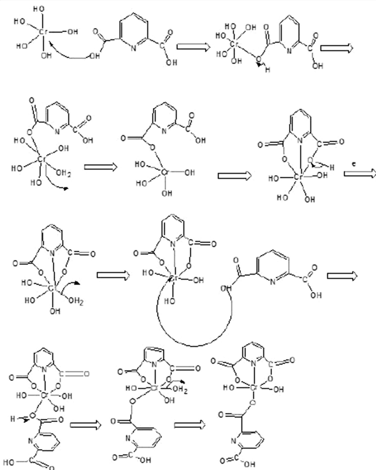
Fig. 3 Proposed mechanism for the formation of Cr-MOF sorbent
