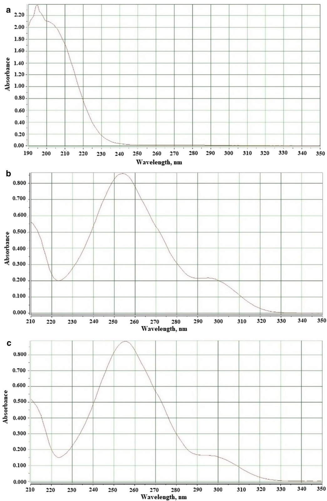
Fig. 8 Absorption spectra of extracted methyl and propyl parabens from wastewater before (a) and after spiking with 85 µg/L of the analytes (b methyl paraben, c propyl paraben)
