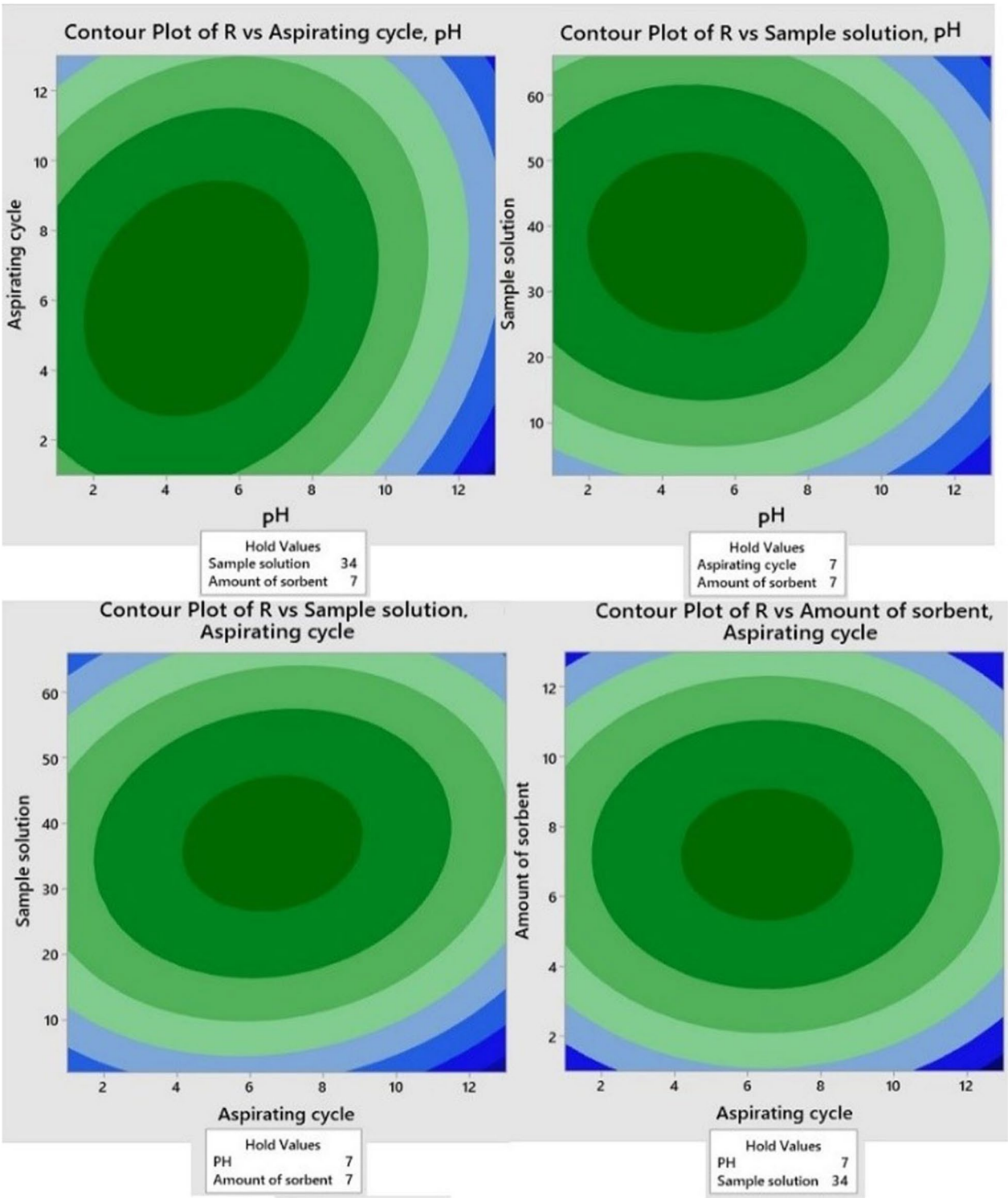
Fig. 6 Response surface-2D/contours explaining the effect of independent variable on response (absorbance) of parabens
