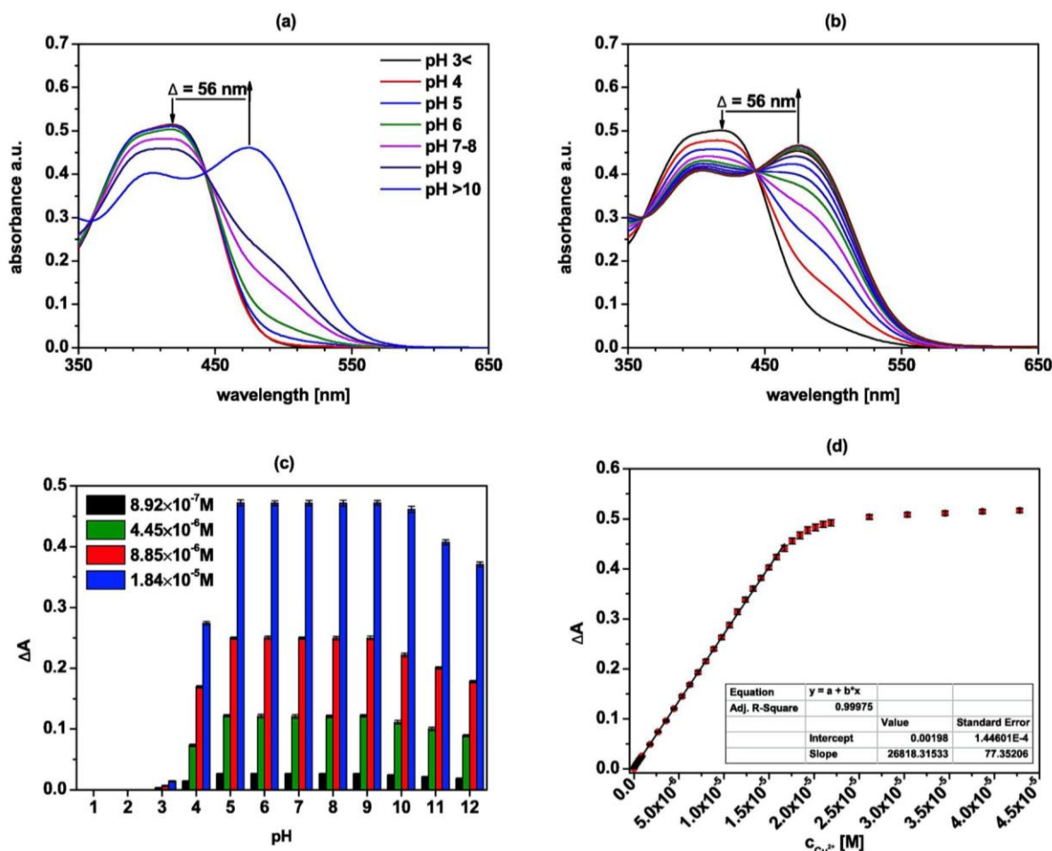
Fig. 14. The change of UV-Vis spectrum of L ( c_L = 2.16 \times 10^{-5} M) (a) with increasing pH and (b) upon titration with sodium hydroxide ( c_{NaOH} = 0-1.08 \times 10^{-5} M) in water-DMSO (9:1, v/v) from pH 6; (c) spectral response towards copper(II) chloride of L ( c_L = 2.16 \times 10^{-5} M) depending on pH ( \lambda = 540 nm); (d) spectral response \Delta A towards copper(II) chloride presence of L ( c_L = 2.16 \times 10^{-5} M) in pH range 5.0–9.0.
