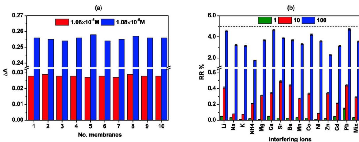
Fig. 22. (a) Reproducibility of optode after contact with copper(II) chloride solution (pH 5.0) and (b) interferences of several metal chlorides used at equimolar, 10-fold and 100-fold molar excess, expressed as RR%, to spectral response ( \Delta A ) of optodes (at 540 nm) towards copper(II) chloride (pH 5.0).
