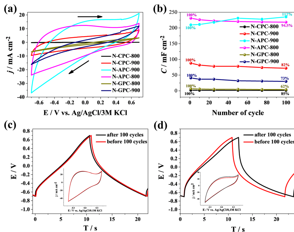
Figure 4. (a) Cyclic voltammetry curves recorded for N-doped carbon materials in 0.2 \text{ mol L}^{-1} \text{ K}_2\text{SO}_4 with a potential window between -0.7 \text{ V} and +0.7 \text{ V} ( \nu = 50 \text{ mV s}^{-1} ). (b) Specific capacitance plotted as a function of cycles for investigated carbon materials. Exemplary galvanostatic charge–discharge curves for N-APC-800 and (d) N-APC-900, recorded at 5 \text{ A g}^{-1} (inset: cyclic voltammetry curves recorded in 0.2 \text{ mol L}^{-1} \text{ K}_2\text{SO}_4 ( \nu = 50 \text{ mV s}^{-1} )).
