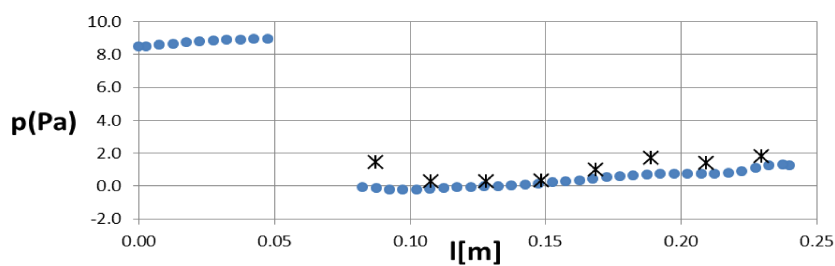
Fig. 9. Numerical and experimental results, path 5, case 1
