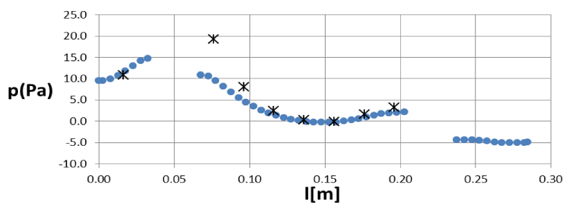
Fig. 10. Numerical and experimental results, path 6, case 1
