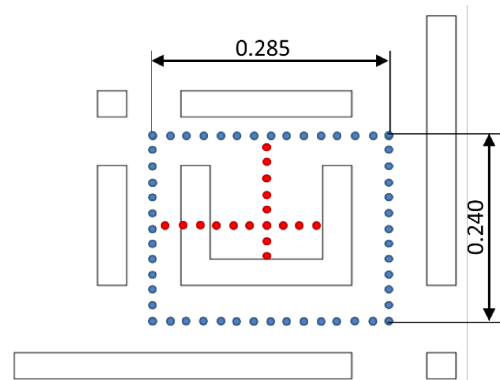
Fig. 3. Positions of pressure sensors (XY plane, dimensions of the model in meters)
