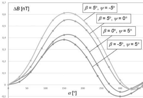
Fig. 7. Disturbances in the magnetic flux density for four selected angles of the sensor
