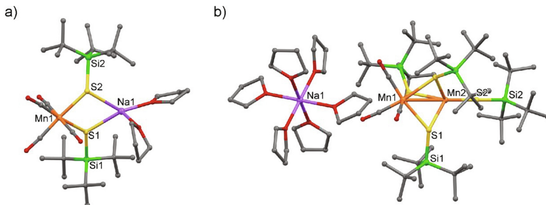
Fig. 17. Molecular structures of the heteroleptic tri- tert -butylsilylanethiolate complexes of Mn(I)/(II) without hydrogen atoms: a) [\text{Na}(\text{THF})_2(\text{OC})_4\text{Mn}(\mu\text{-Si}t\text{-Bu}_3)_2] [120]; b) [\text{Na}(\text{THF})_6][(\text{OC})_3\text{Mn}(\mu\text{-Si}t\text{-Bu}_3)_3\text{MnSi}t\text{-Bu}_3] [120].
