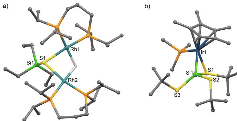
Fig. 33. Molecular structures of ruthenium and iridium silanethiolates; hydrogen atoms are omitted for clarity: a) [\text{Rh}_2(\mu\text{-H})(\mu\text{-SSiEt}_3)(\text{dipp})_2] [173]; b) [\text{Cp}^*(\text{PMe}_3)\text{Ir}(\kappa^2\text{-Si}(\text{SrBu})_2\text{SrBu})[\text{OTf}]] [174].
