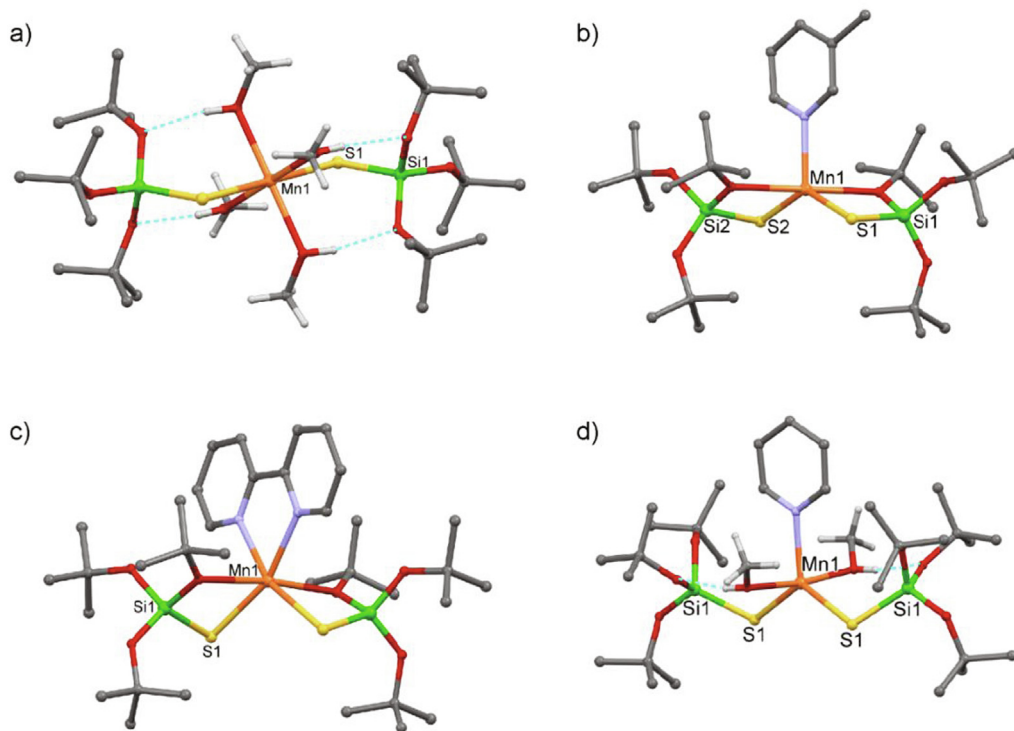
Fig. 15. Molecular structures of the heteroleptic tri- tert -butoxysilanethiolate complexes of Mn(II) H atoms of the t Bu groups and pyridine ligands are omitted for clarity: a) [(MeOH) 4 Mn{SSi(O t Bu) 3 } 2 ] [115]; b) [(3- Mepy )Mn{SSi(O t Bu) 3 } 2 ] [117]; c) [(2,2'- bipy )Mn{SSi(O t Bu) 3 } 2 ] [116]; d) [(MeOH) 2 ( py )Mn{SSi(O t Bu) 3 } 2 ] [117].
