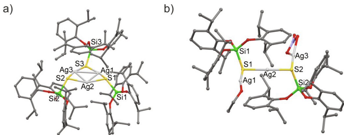
Fig. 47. Molecular structures without hydrogen atoms of the trinuclear Ag(I) complexes with the (\text{dippO})_3\text{SiSi}^- ligand: a) [\{\text{Ag}(\text{SSi}(\text{Odipp})_3)\}_3] ; b) [(\text{EtOH})\text{Ag}_3(\text{NO}_3)\{\mu\text{-SSi}(\text{Odipp})_3\}_2] [52].
