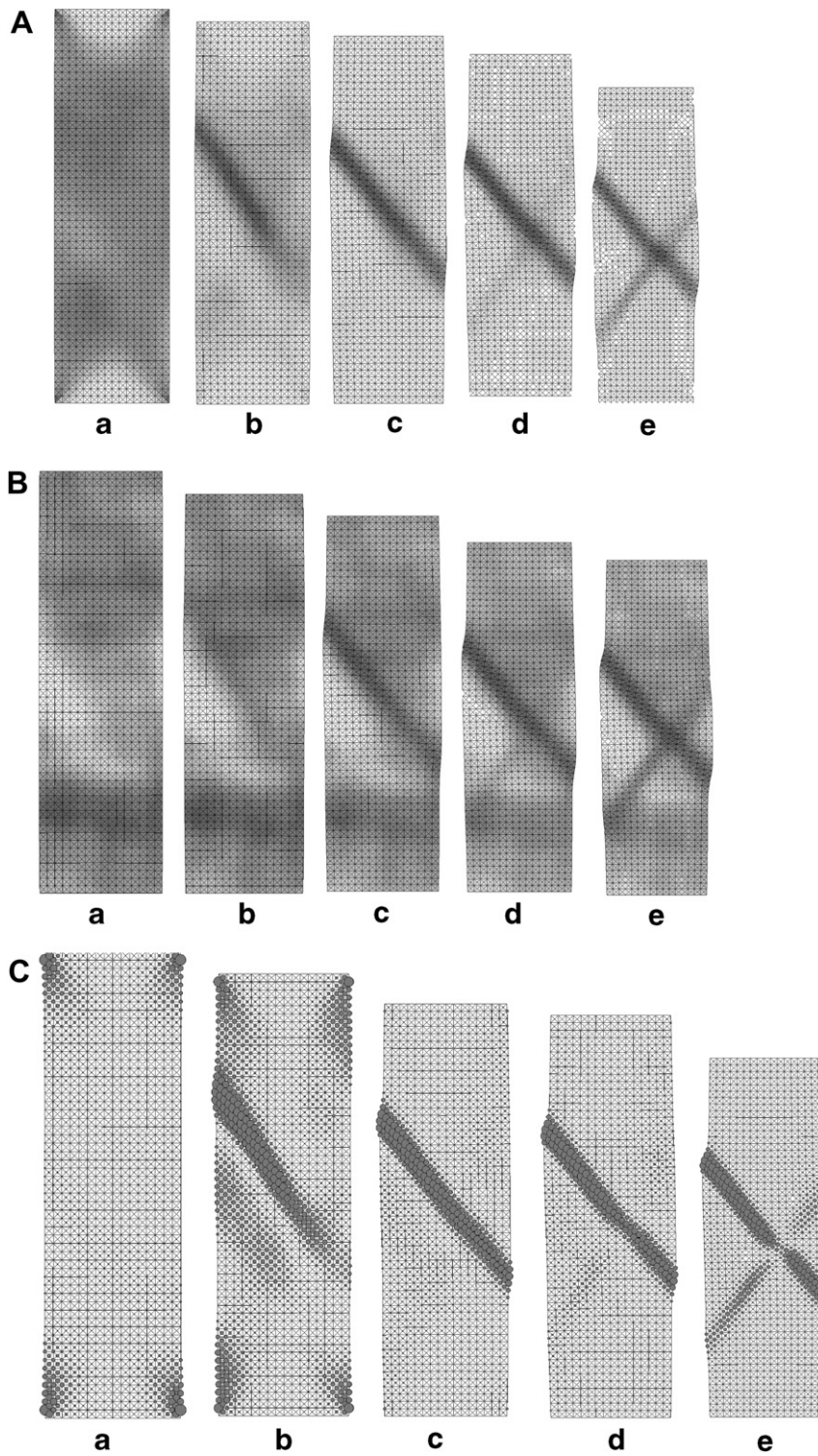
Fig. 16. Evolution of equivalent total strain measure (A), void ratio (B) and Cosserat rotation (C) field during a plane strain compression test (random field of Fig. 13d) at: (a) u_2/h_0 = 0.011 , (b) u_2/h_0 = 0.021 , (c) u_2/h_0 = 0.028 , (d) u_2/h_0 = 0.036 , (e) u_2/h_0 = 0.042 ( \bar{e}_0 = 0.60 , very rough boundaries, specimen size 40 \times 140 \text{ mm}^2 ).
