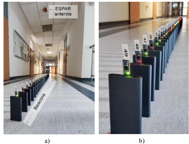
Fig. 1. Test setup arranged for the measurements: a) Test configuration overview; b) Beacons spaced at equal intervals of 10 cm.
