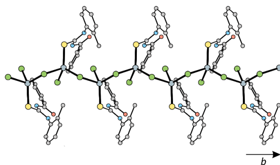
Figure 13. Coordination polymer chain with pc11 rod symmetry in structure of 4 . Hydrogen atoms and solvent molecules are omitted for clarity.
