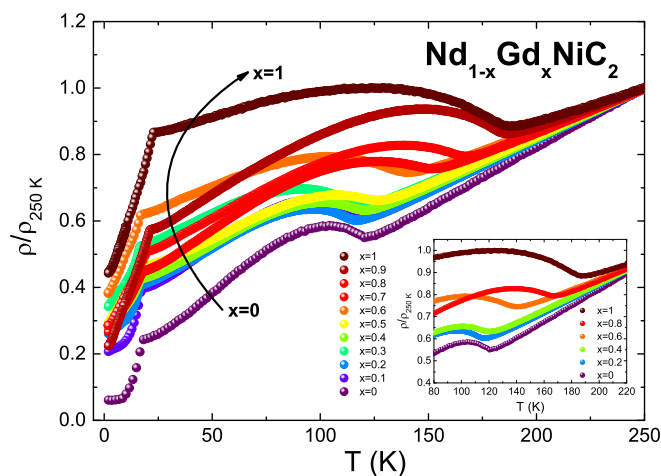
FIG. 2. Temperature dependence of the normalized electrical resistivity \rho/\rho_{250\text{K}}(T) for \text{Nd}_{1-x}\text{Gd}_x\text{NiC}_2 ( 0 \leq x \leq 1 ). Inset shows the vicinity of the CDW transition for selected samples for better clarity.
