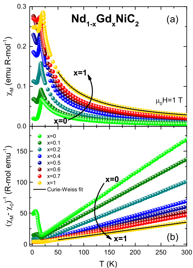
FIG. 3. Temperature dependence of the molar magnetic susceptibility \chi_M (a) and of the reciprocal molar magnetic susceptibility (\chi_M - \chi_0)^{-1} (b) for selected samples from the \text{Nd}_{1-x}\text{Gd}_x\text{NiC}_2 ( 0 \leq x \leq 1 ) series.
