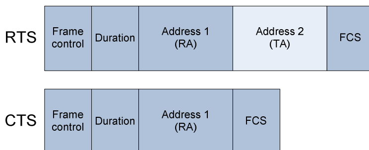
Fig. 8 RTS/CTS Control frames
