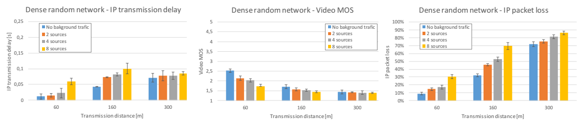
Fig. 85 Impact of background traffic on a non-interactive video transmission in different (A – sparse grid, B – dense grid, C – sparse random, D – dense random) structures of IEEE 802.11 MBSS network
