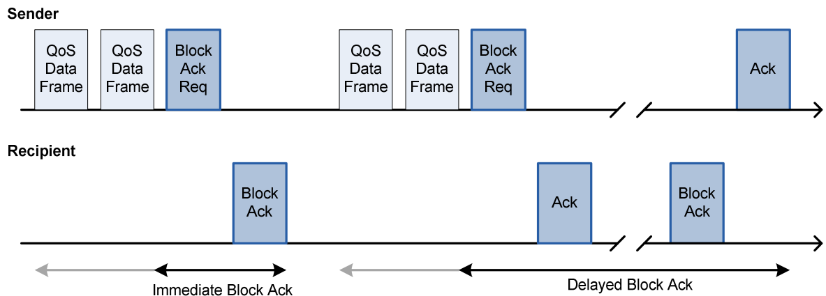
Fig. 17 Block Acknowledgement procedure.
