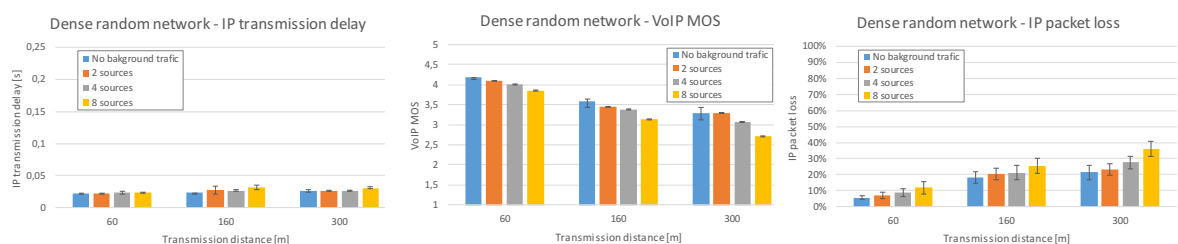
Fig. 84 Impact of background traffic on a VoIP transmission in different (A – sparse grid, B – dense grid, C – sparse random, D – dense random) structures of IEEE 802.11 MBSS network
