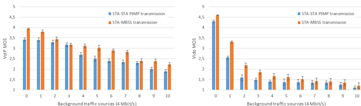
Fig. 80 MOS values for STA-STA transmissions between neighboring STAs in IEEE 802.11 PtMP and IEEE 802.11s MBSS networks (left chart – VoIP, right chart – video)
