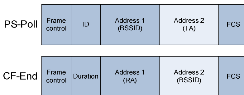
Fig. 10 PS-Poll and CF-End Control frames
