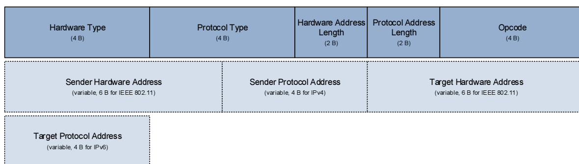
Fig. 91 Address Resolution Protocol message format
