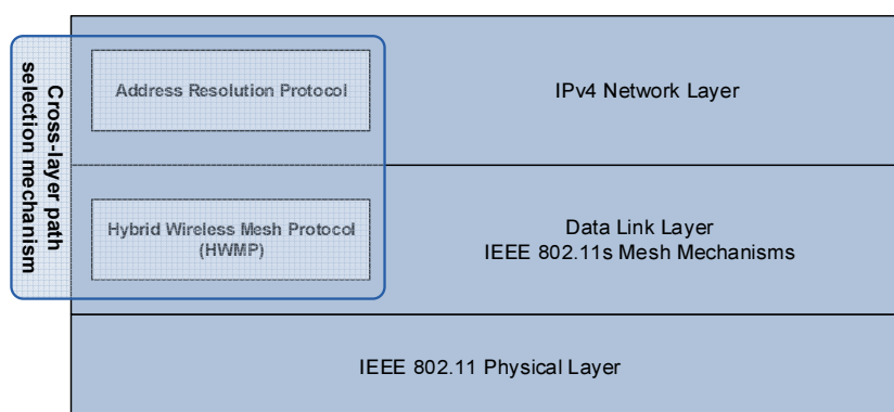
Fig. 92 Cross-layer address resolution procedure placement in ISO-OSI model
