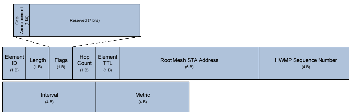
Fig. 72 Root Announcement (RANN) Information Element
