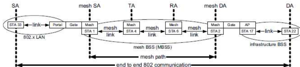
Fig. 54 Mesh address types and their significance areas
