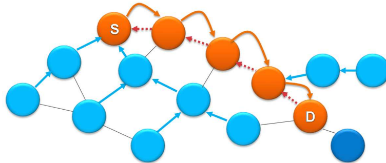
Fig. 71 RM-AODV forward path formation
