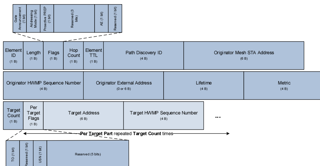
Fig. 68 Path Request (PREQ) Information Element
