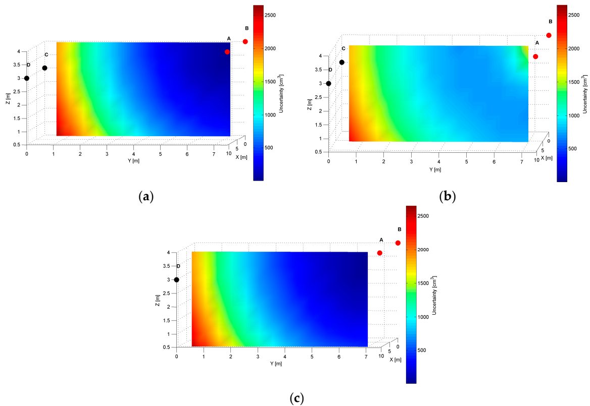
Figure 12. Cross-section ( YZ plane) plots of uncertainty-precision distribution for location sensors A and B at (a) x = 1.00 \text{ m} ; (b) x = 5.50 \text{ m} ; (c) x = 10.00 \text{ m} .
