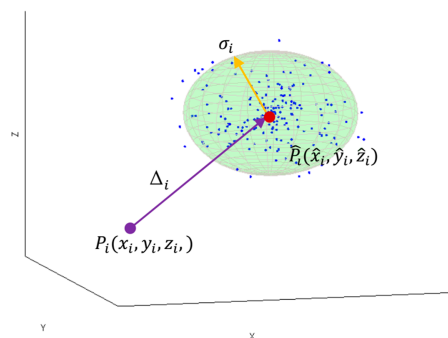
Figure 1. Illustration of 3D localization accuracy and precision for i -th tag's position.
