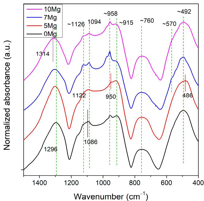
Figure 3. FTIR spectra for all samples.
