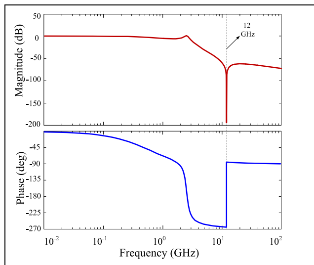
FIGURE 4. The Bode plot of the extracted transfer function.
