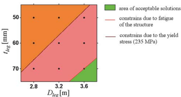
Fig. 14. Area of acceptable solutions with constraints for the structure with leg spacing radius r_{leg} = 25\text{ m} . Node 1.
